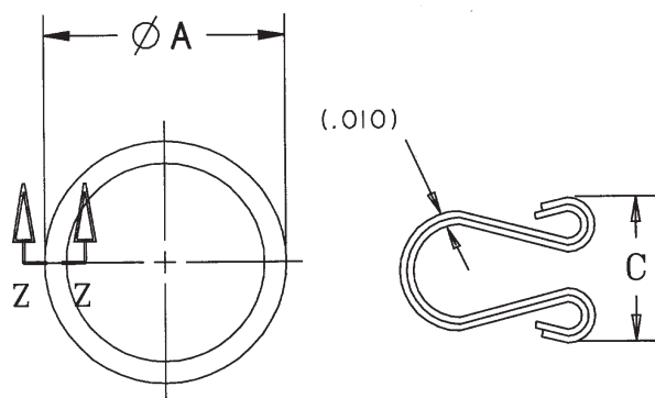
SECTION Z-Z
