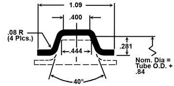
Retainer Gauge: .080 Band Gauge and Width: .063 x 1.000
